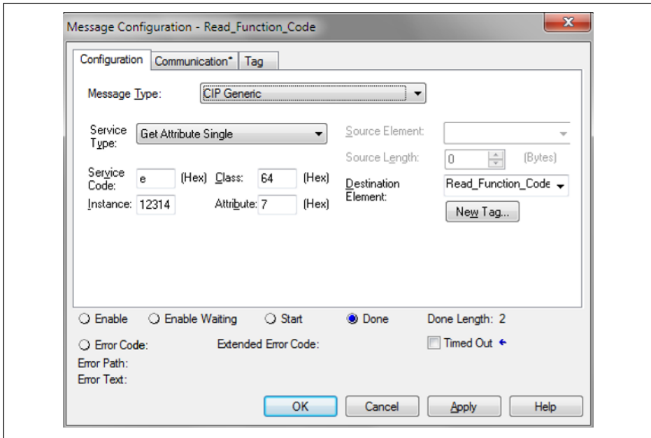
Fig. 6-9: Message configuration
