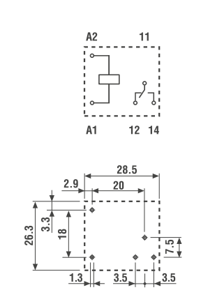
Copper side view Pin length 3.5 mm for PCB
