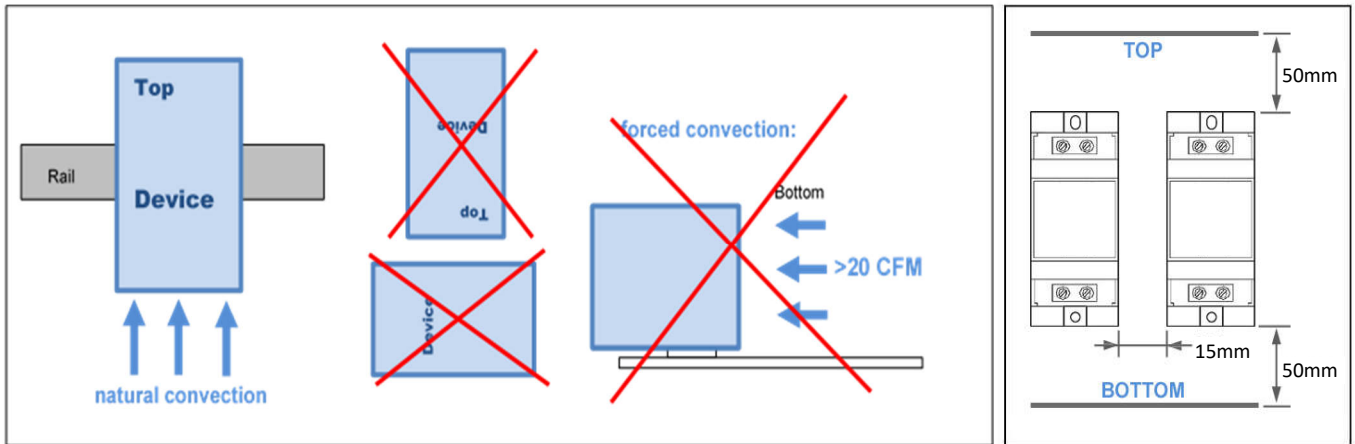
Mounting Instruction: recommended airflow space below and above is 50mm (2 Inch)
