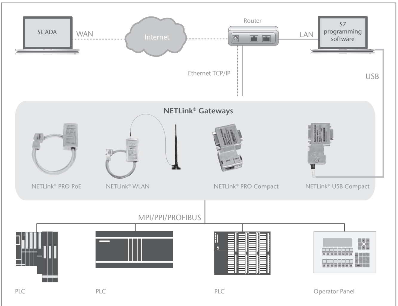
Application example for LAN-WAN connection via ISO on TCP
