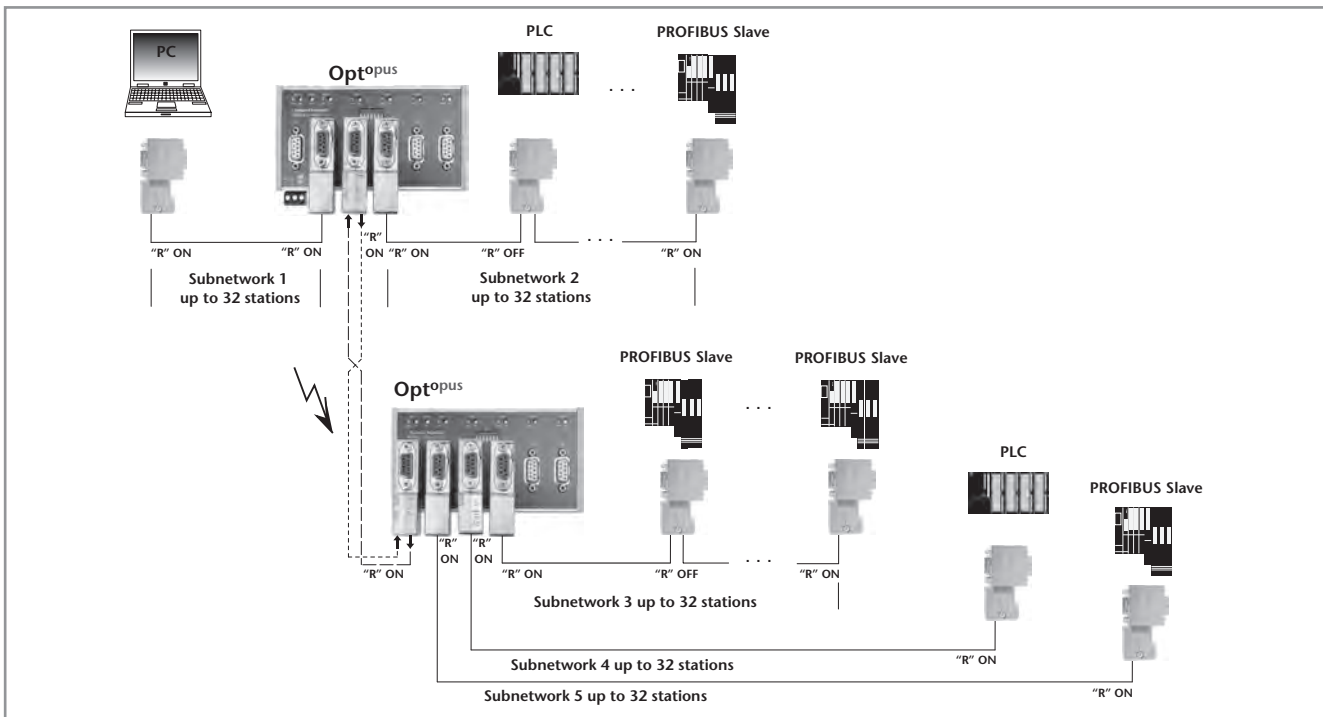
Establish a connection between two repeaters without being influenced by EMI interference.
