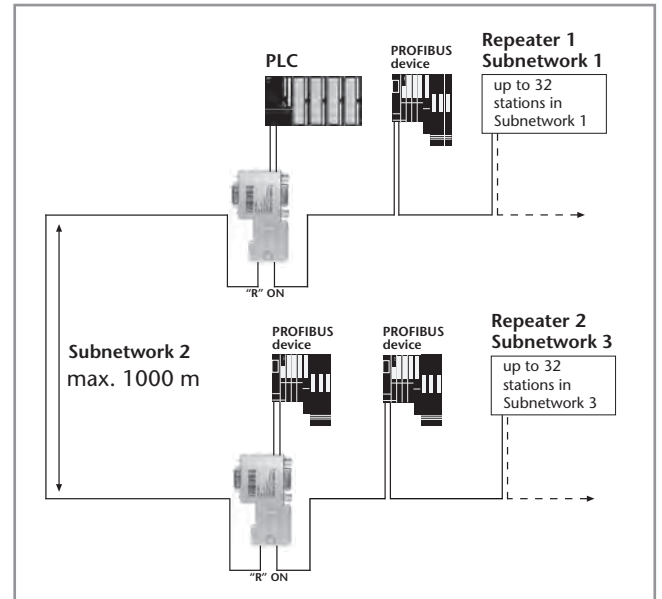
Application example long distance
