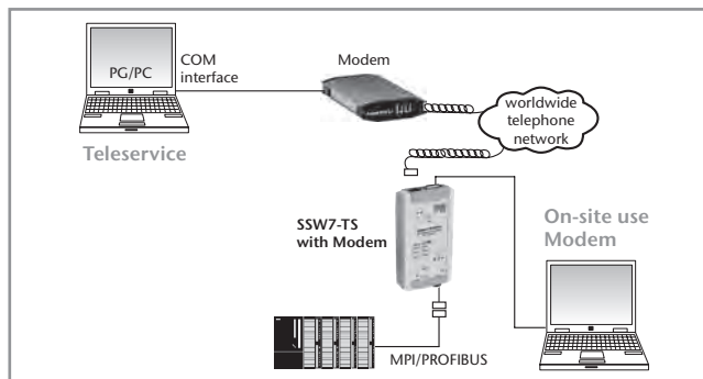
Application example for SSW7-TS with analog modem
