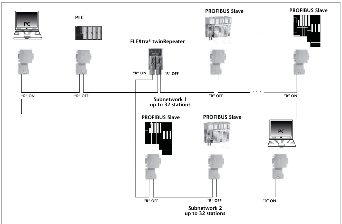
Application example FLEXtra ® twinRepeater stub
