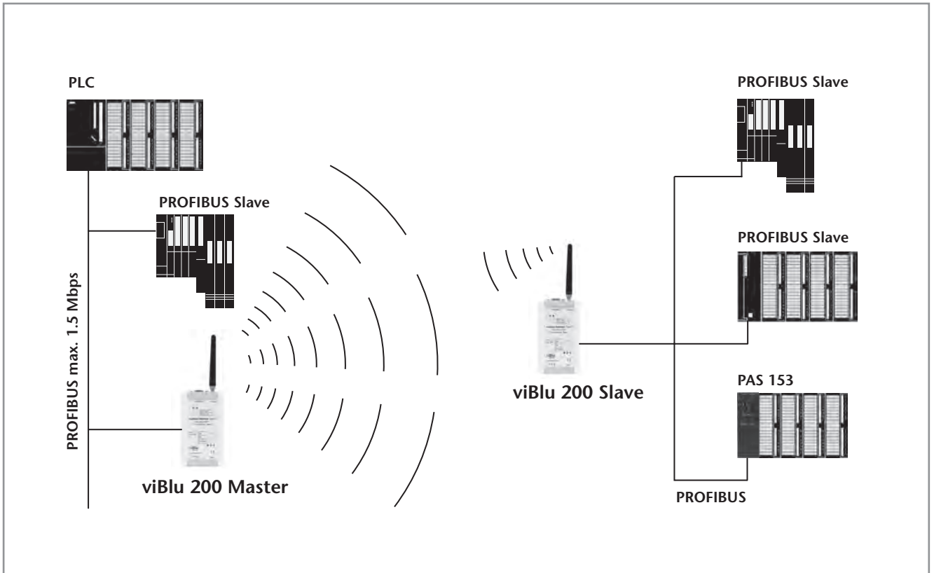
Application example viBlu 200 with a radio slave and up to three PROFIBUS-DP participants
