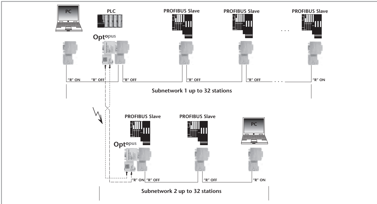
Generate a SUB network that is fully isolated electrically.
