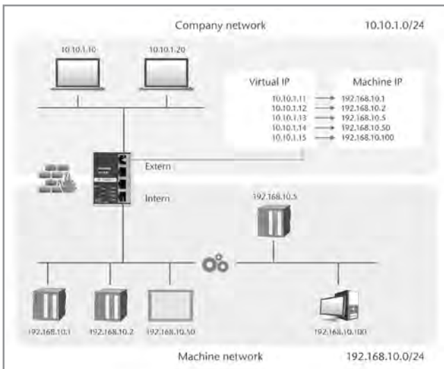
WALLIE, Basic NAT
