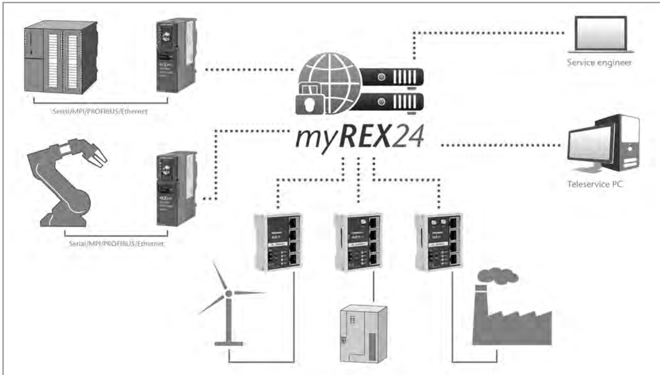
Functional principle of myREX24
