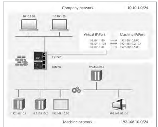
WALLIE, NATP: Network Address and Port Translation
