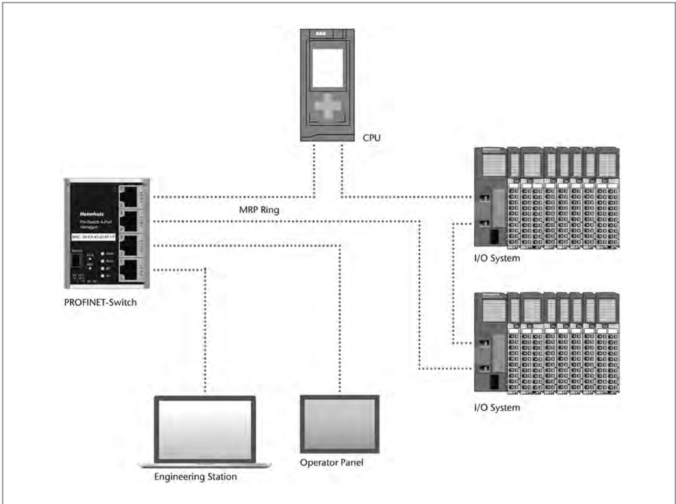
Application example for PROFINET Switch, 4-port, managed
