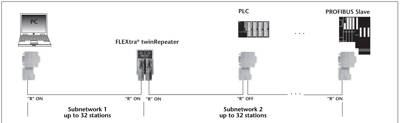
Application example of FLEXtra ® twinRepeater with more than 32 participants
