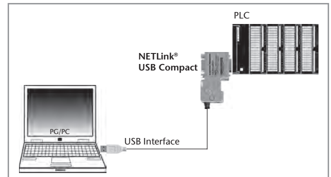
Application example for NETLink® USB Compact
