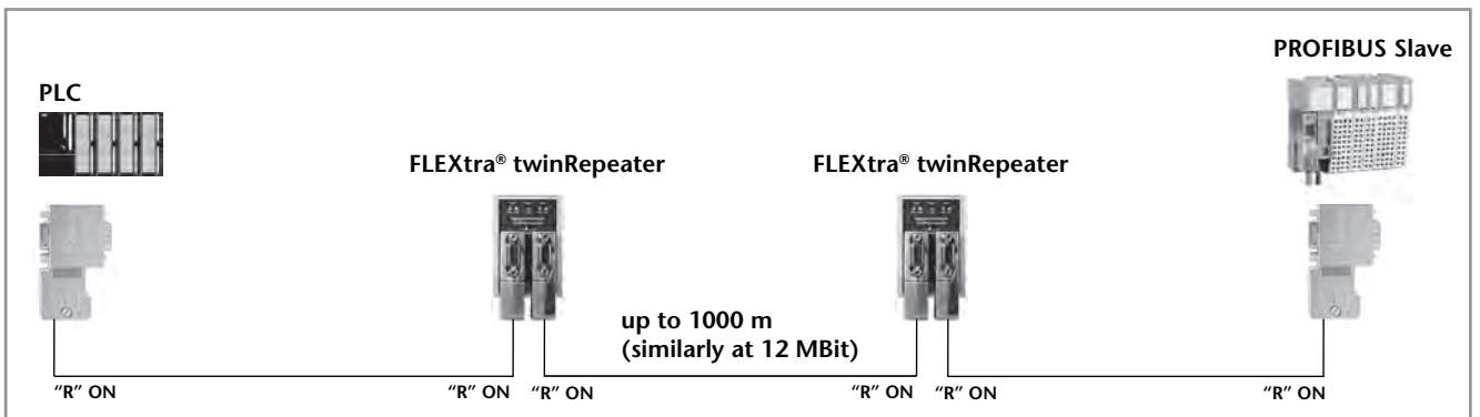
Application example FLEXtra ® twinRepeater long distance
