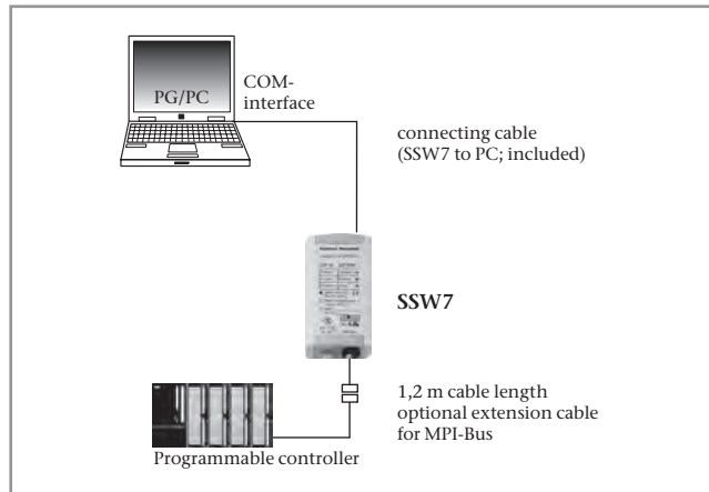
Application example for SSW7
