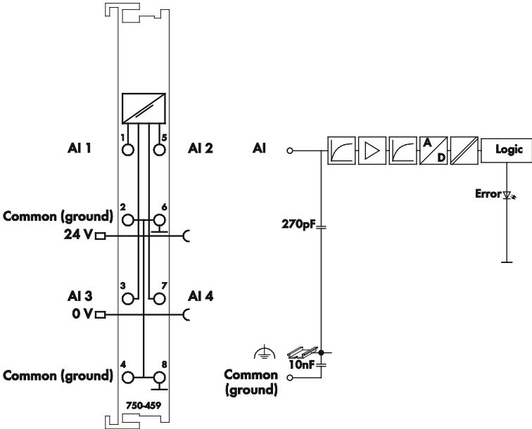
Figure 6: Schematic Diagram
